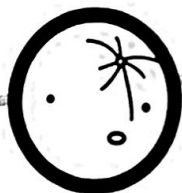
Mercury
